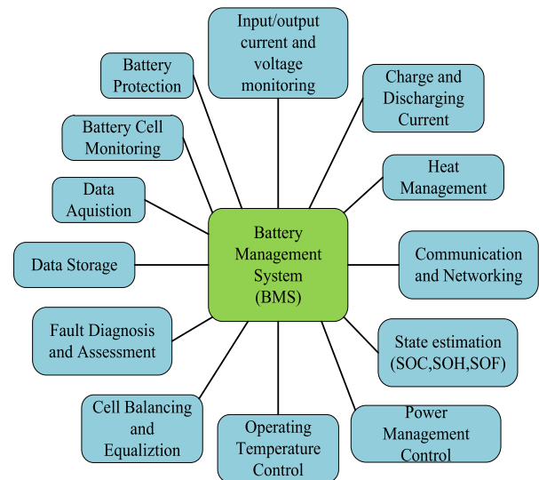
FIGURE 38. Summary of Battery management system.
