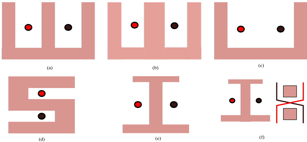
FIGURE 21. Power rail basic shapes (a) E-type. (b) W-type. (c) U-type. (d) S-type. (e) I-type. (f) Cross-segmented structure.
