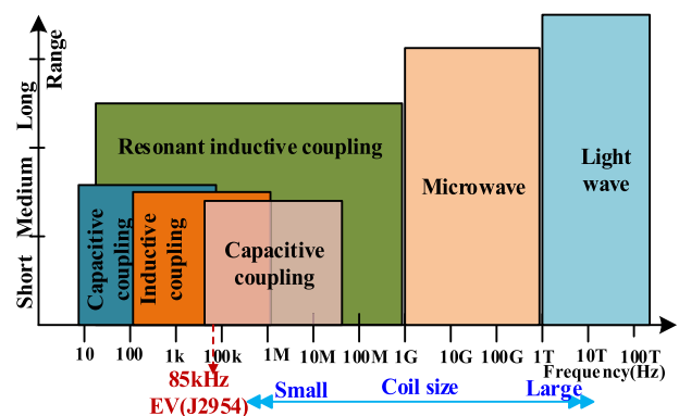
FIGURE 7. Operation range and frequency of different WPT methods.
