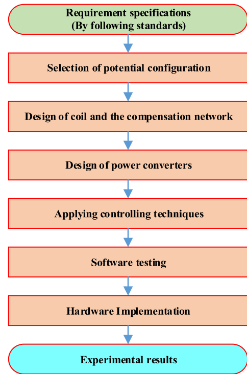
FIGURE 15. Flow chart: design procedure of a WPT.
