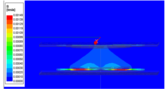
FIGURE 44. Flux distribution in the Ansys-Maxwell FEA model.
