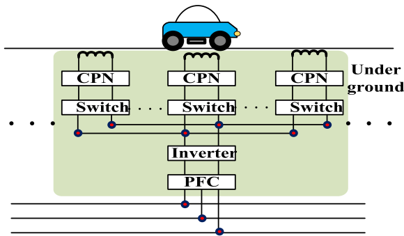
FIGURE 35. HF inverter feeding multiple modules.
